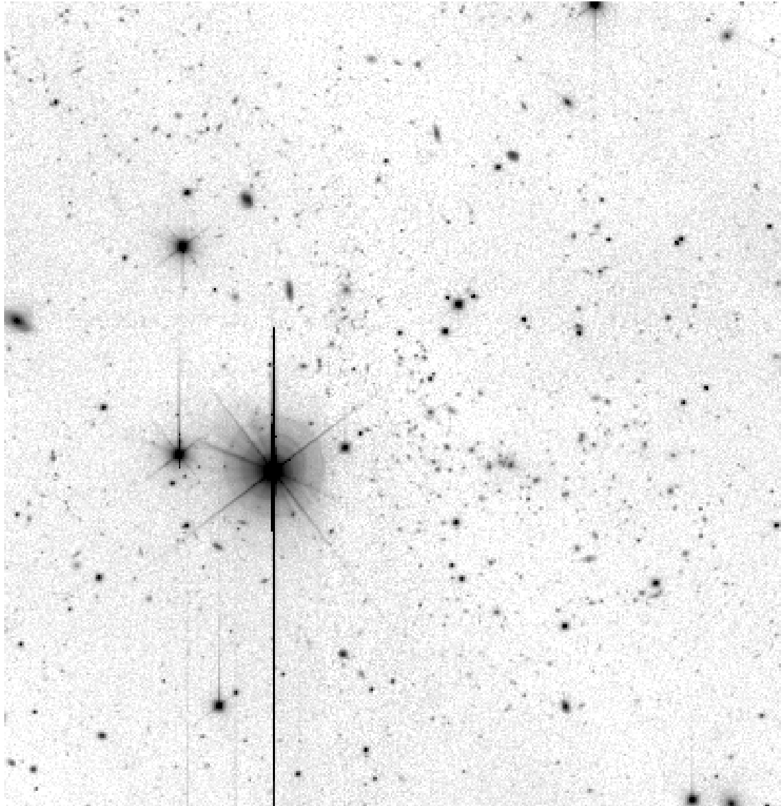
Figure 2: Subarray I image of the NEP cluster RXJ1716+66 at z = 0.81 taken with the University of Hawai'i \times 8K CCD mosaic camera on the CFHT prime focus
