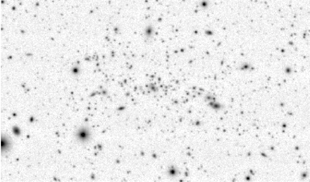
Figure 1: Subarray I image of MS 1054–03 at z = 0.83 taken with the Tek 2048 CCD camera at the University of Hawai'i 2.2m
