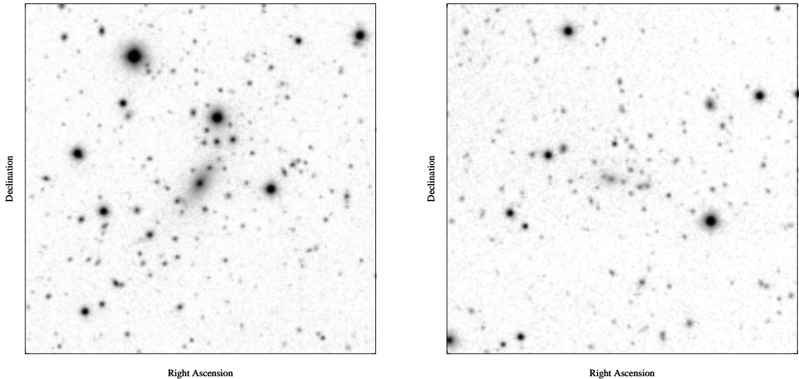
Figure 3: R band images of MACS clusters obtained with the University of Hawaii's 2.2m telescope. Left: one of the most nearby and least X-ray luminous clusters in the MACS sample ( z = 0.329 , L_X = 6.4 \times 10^{44} erg s ^{-1} , 0.1–2.4 keV). Right: One of the most distant and more X-ray luminous clusters in the MACS sample ( z = 0.570 , L_X = 1.7 \times 10^{45} erg s ^{-1} , 0.1–2.4 keV). Both clusters are new discoveries. The shown images span 1 h_{50}^{-1} Mpc on the side at the cluster redshift.
